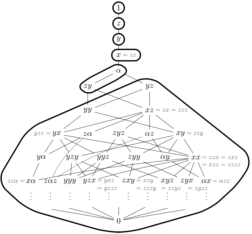
Figure 1: The free one-element coextension \mathcal{R}(S) for the tomonoid S from Example 3.7 and a coextension congruence.
