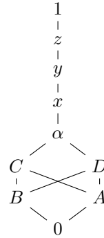
Figure 3: The free one-element (1, 1) -coextension \mathcal{R}_{1,1}(S) discussed in Example 4.6. Here, S is the tomonoid from Example 3.7.
